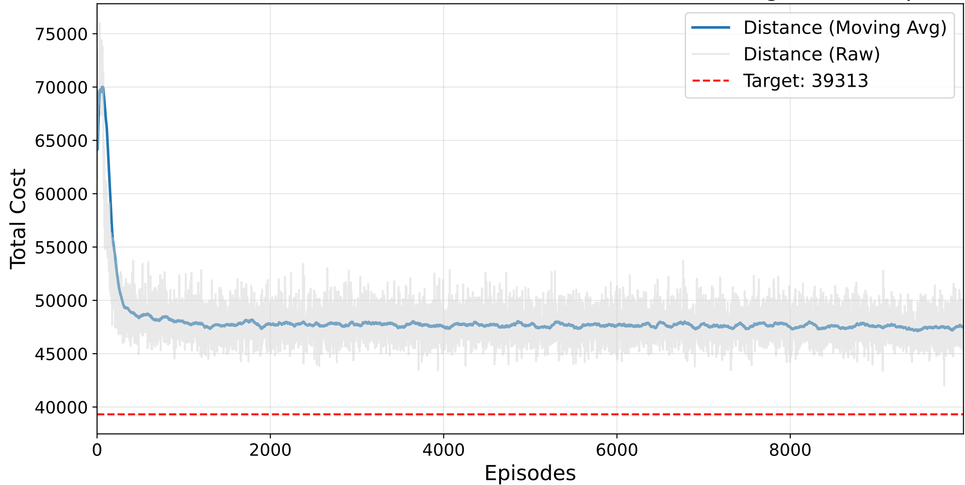
Final GAUSSIAN PROCESS Masked AutoRL-SOP Training - ft70.1.sop
